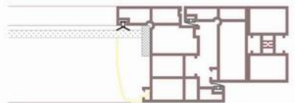
DETAIL KUSEN PJ-Z
